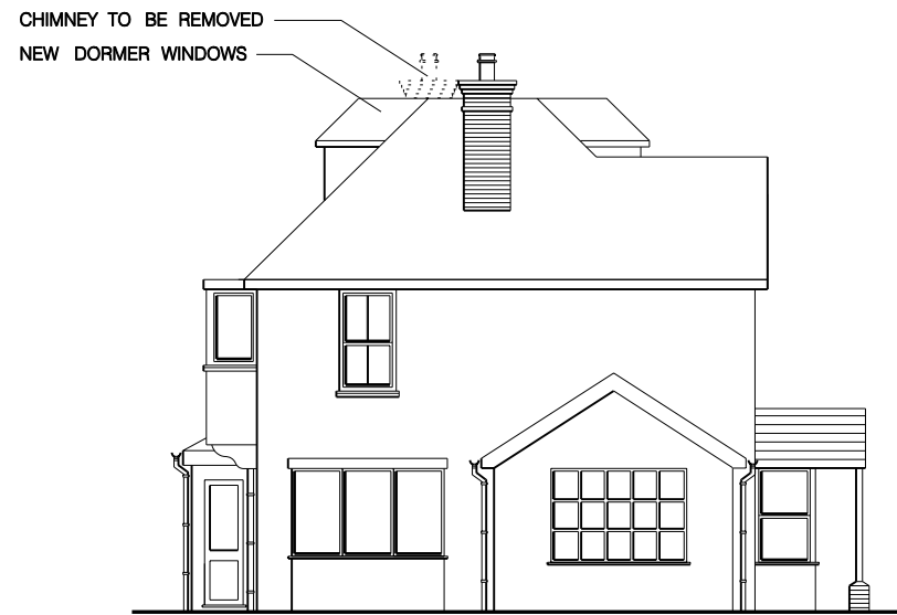
SIDE ELEVATION
